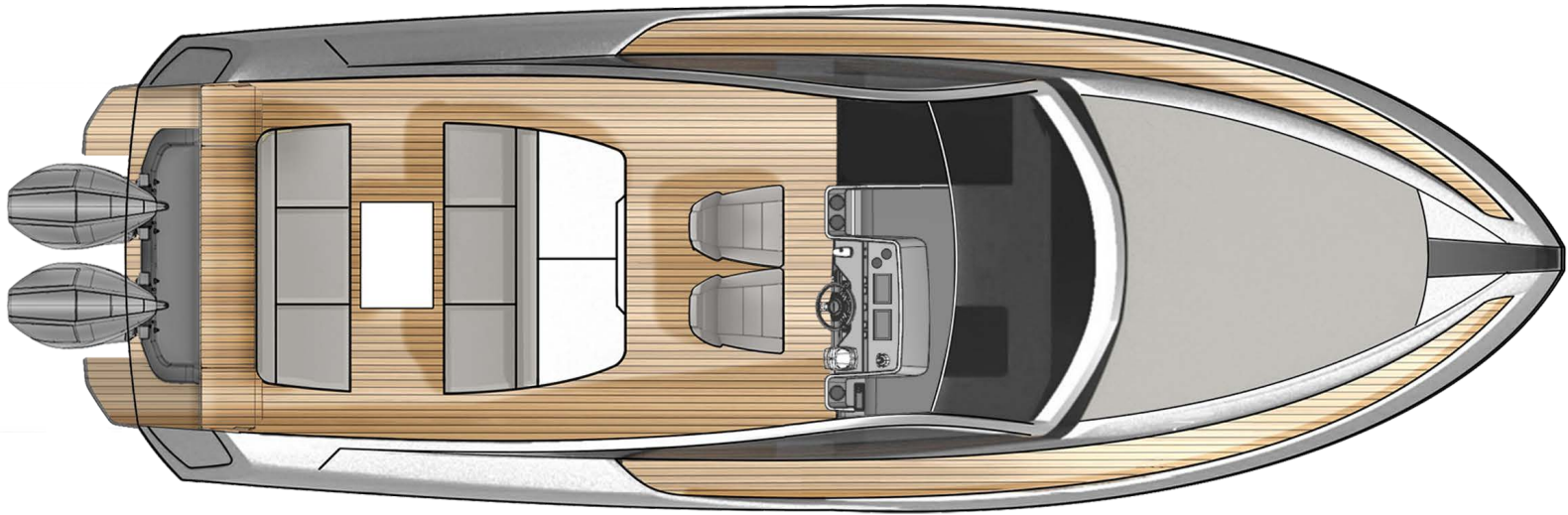
COCKPIT LAYOUT 1
